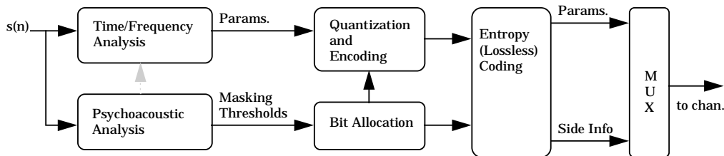
Fig. 1. Generic Perceptual Audio Encoder
