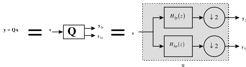
Fig. 23. Filter Bank Interpretation of the DWT
