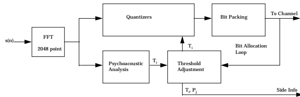
Fig. 19. PXFМ Encoder (after [6])
